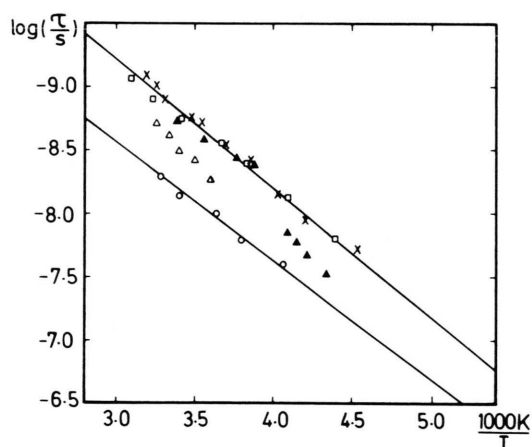
Fig. 4. Arrhenius plots of the label fluctuations: ( \square ), crystallized metHb-Mal5, S_2(0) = 0.78 ; ( \circ ), lyophilized metHb-Mal5, W\% = 16.3 , S_2(0) = 0.78 ; ( \times ), crystallized metHb-Mal6, S_2(0) = 0.73 ; ( \triangle ), metHb-JAA6 in viscous solution ( \tau determined from the outer hyperfine separation using Eqn. (7) and (2) with S_2(0) = 0.73 ); and ( \blacktriangle ), free Tempone radicals in metHb single crystal, \tau determined from the calibration curve for isotropic rotational diffusion given in Fig. 3.
