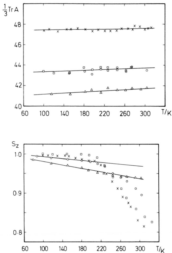
Fig. 1. a) The trace of the hyperfine tensor, 1/3 \text{Tr} A , as a function of temperature of spin-labeled methemoglobins: ( \square ) crystallized metHb-Mal5; ( \triangle ), lyophilized metHb-Mal5, degree of hydration W\% = 0 ; ( \circ ), lyophilized metHb-Mal5, W\% = 16.3 ; ( \times ) crystallized metHb-Mal6. b) The parameter S_z as a function of temperature for the samples shown in a). The lines are the best fits of the torsional oscillation model to the lyophilized metHb-Mal5 data.
