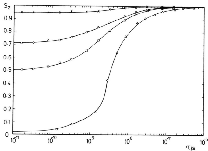
Fig. 3. The parameter S_z versus correlation time for the two-jump model: ( \times ), semiangle \theta = 12.5^\circ ; ( \circ ), \theta = 30^\circ ; ( \square ), \theta = 45^\circ ; and for ( \triangle ) isotropic Brownian diffusion. This curve was determined from fittings of spectra on the basis of the time-independent effective Hamiltonian to spectral simulations using the stochastic Liouville equation [19]. Parameters of the simulations are given in [12].
